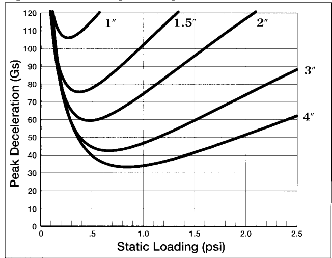
Figure 10 - 36" Drop, 2-5 Impacts
