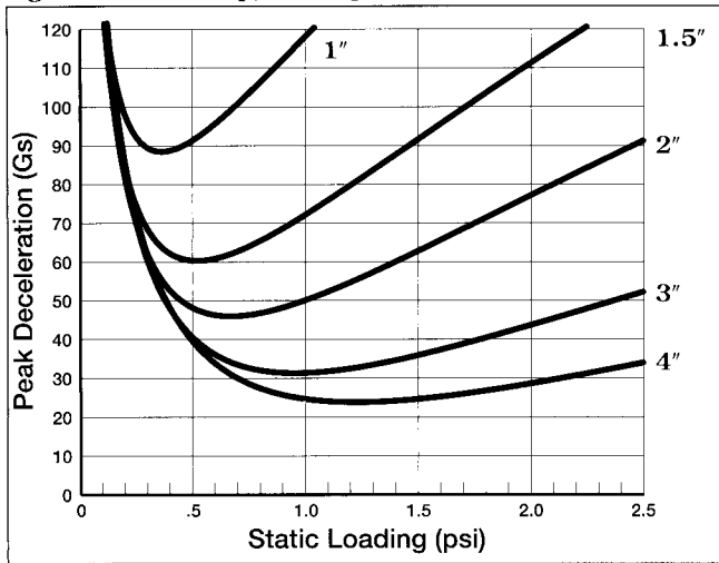
Figure 9 - 36" Drop, 1st Impact
