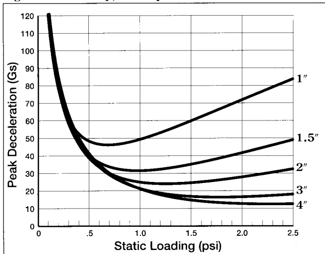
Figure 3 - 18" Drop, 1st Impact
