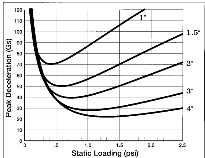
Figure 6 - 24" Drop, 2-5 Impacts
