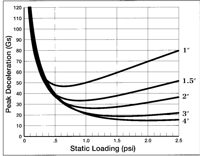
Figure 2 - 12" Drop, 2-5 Impacts
