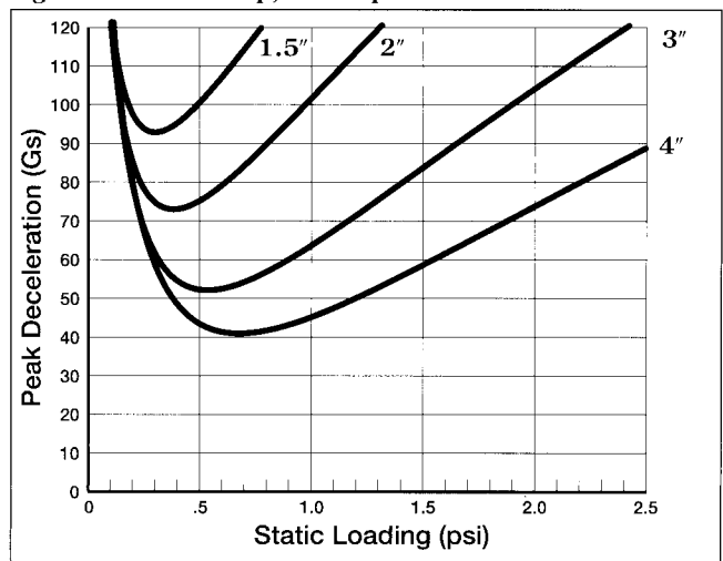
Figure 12 - 42" Drop, 2-5 Impacts
