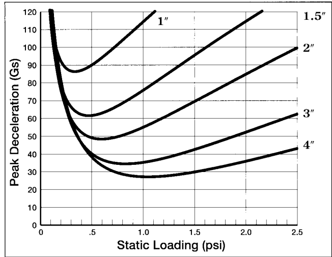
Figure 8 - 30" Drop, 2-5 Impacts
