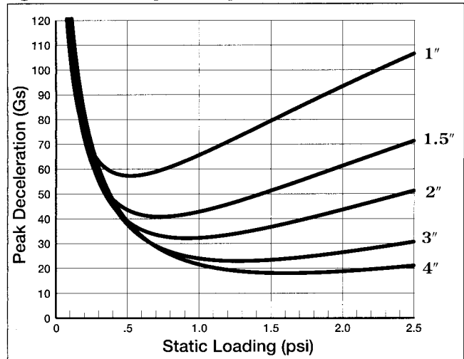
Figure 4 - 18" Drop, 2-5 Impacts
