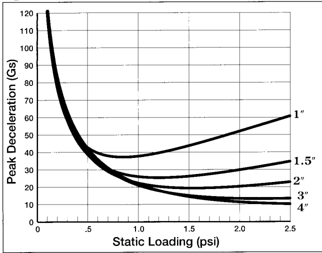
Figure 1 - 12" Drop, 1st Impact
