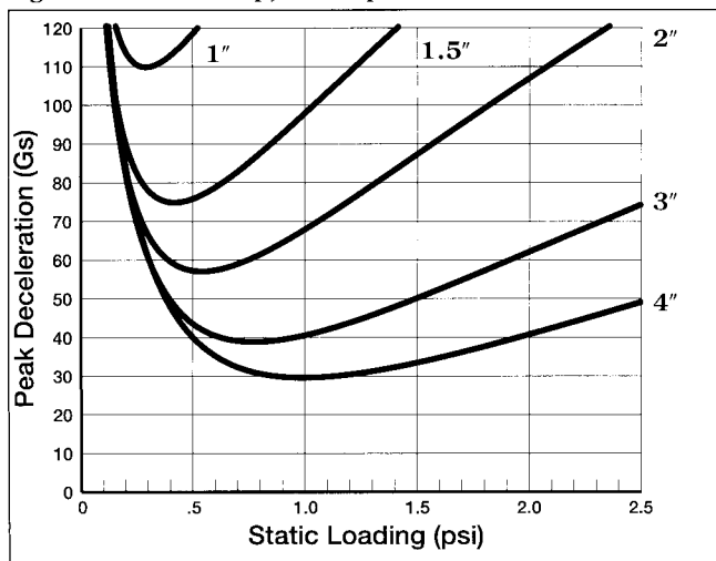
Figure 11 - 42" Drop, 1st Impact
