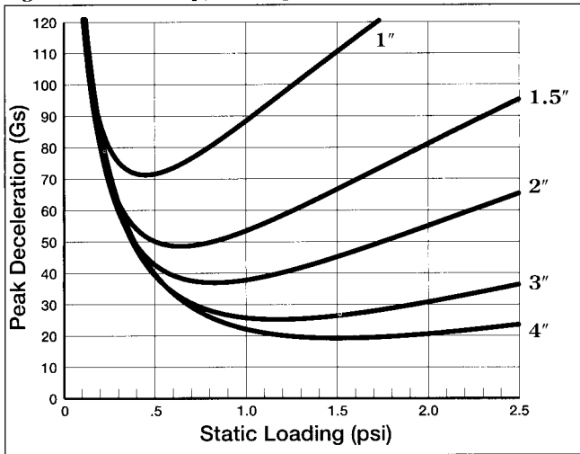
Figure 7 - 30" Drop, 1st Impact
