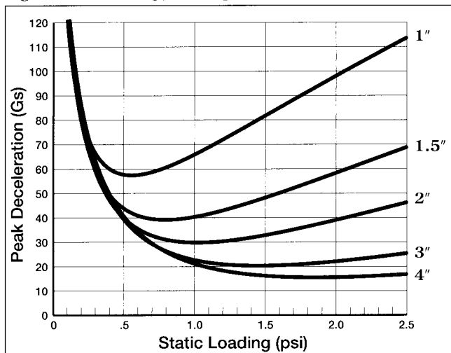
Figure 5 - 24" Drop, 1st Impact
