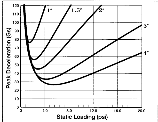
Figure 8 - 24" Drop, 2-5 Impacts
