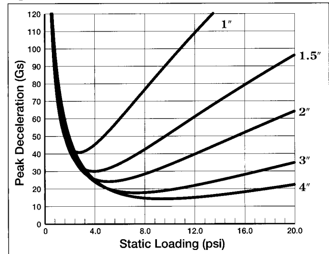
Figure 4 - 12" Drop, 2-5 Impacts
