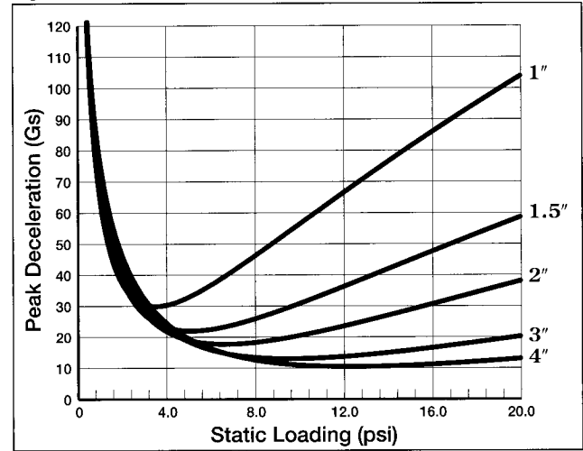
Figure 2 - 6" Drop, 2-5 Impacts
