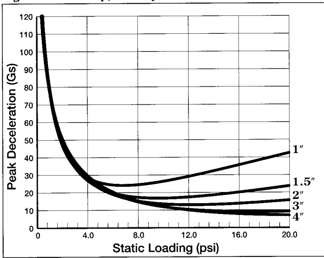
Figure 1 - 6" Drop, 1st Impact
