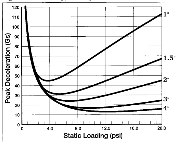
Figure 5 - 18" Drop, 1st Impact
