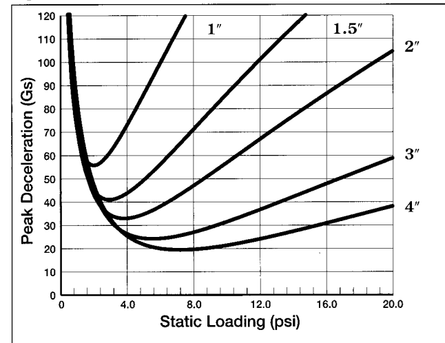
Figure 6 - 18" Drop, 2-5 Impacts
