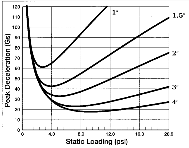
Figure 7 - 24" Drop, 1st Impact
