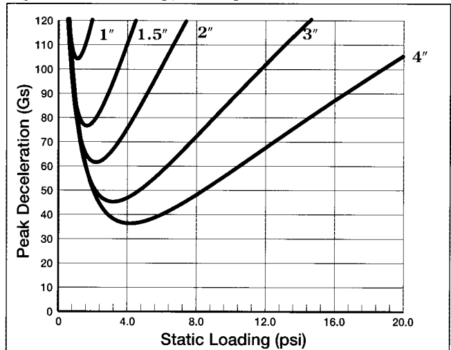
Figure 10 - 30" Drop, 2-5 Impacts
