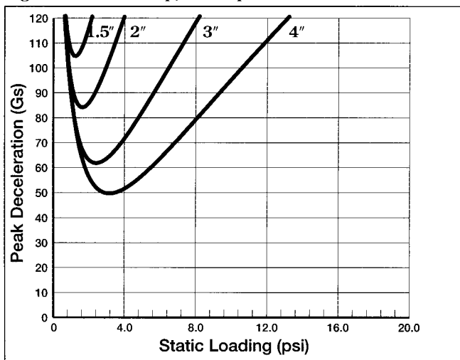
Figure 11 - 36" Drop, 1st Impact
