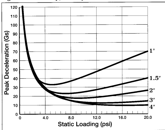
Figure 3 - 12" Drop, 1st Impact
