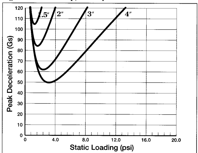
Figure 12 - 36" Drop, 2-5 Impacts
