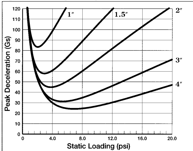
Figure 9 - 30" Drop, 1st Impact
